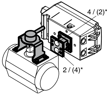
Mounting: NAMUR adapter V Control air connector code -V-
