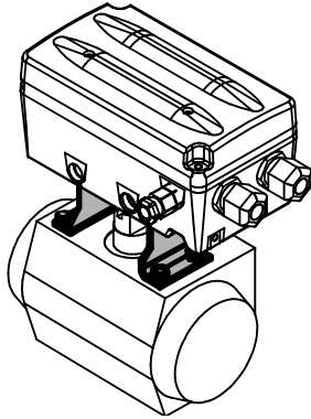
Mounting: Mounting bracket Control air connector code 000
